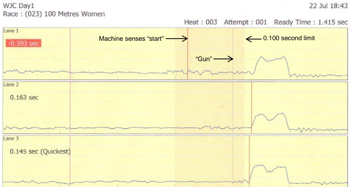
Figure 13: A false start indication that is false
